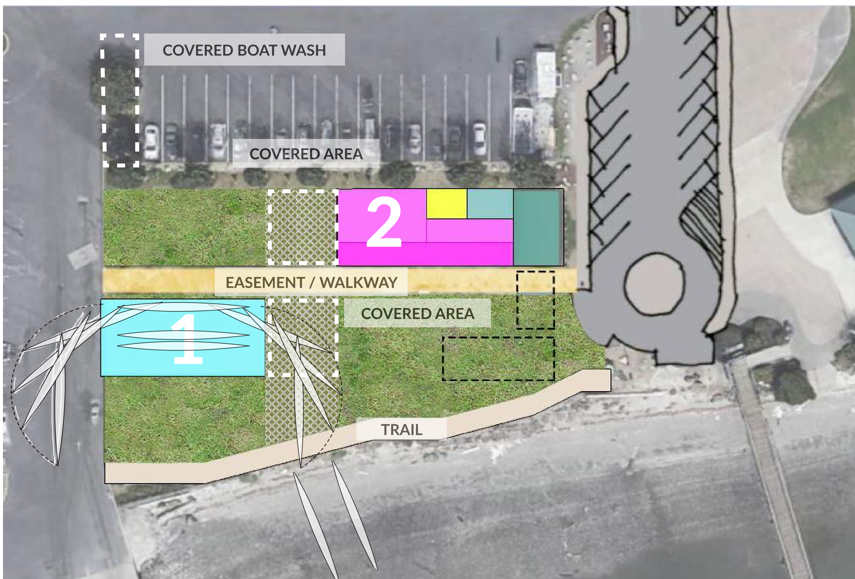
SITE PLAN
